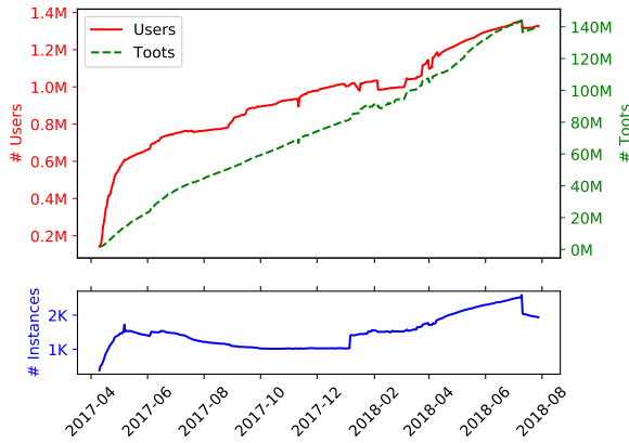
Figure 1: Available instances/user/toots over-time.
