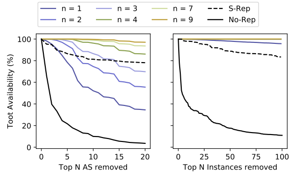
Figure 16: Availability of toots when removing top instances (measured by #toots) with random replication. Lines for n > 4 overlap indicating availability above 99% (97%) in case of instance (AS) failures.
